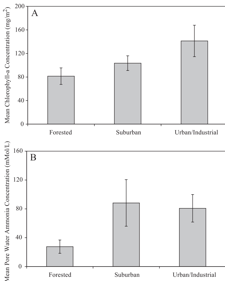
Fig. 4. The mean surface sediment chlorophyll a (A) and pore water ammonia (B) concentrations in 2000 winter calibration study for each watershed type. Error bars represent \pm 1 standard error.
