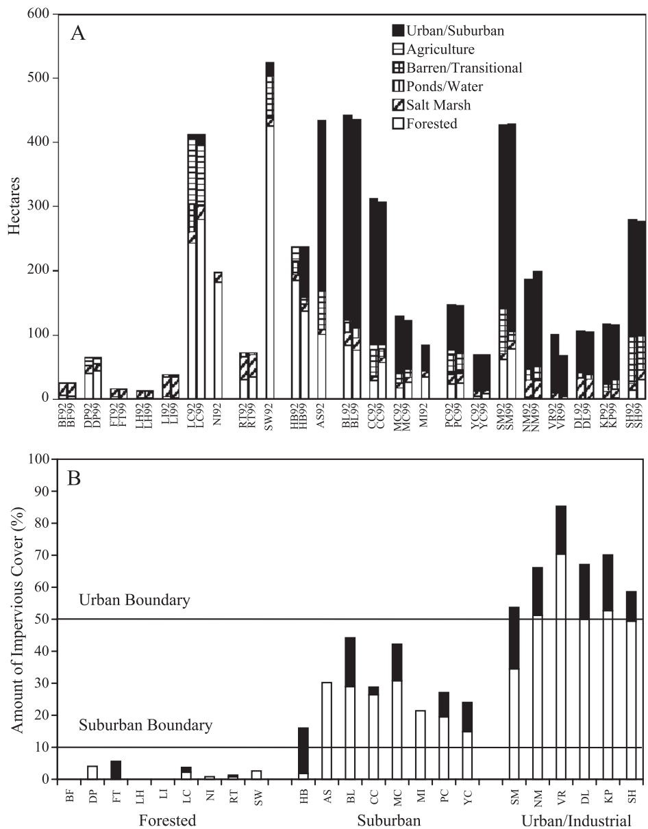
Fig. 2. Summary of land cover and watershed size for each creek based upon 1992 and 1999 aerial photographs (A). The amount of impervious cover in the watersheds for the 1992 aerial photographs (white) and the increase in impervious cover between 1992 and 1999 (shaded) (B). The creek abbreviation (see Table 1) and photograph year are presented along the x-axis.
