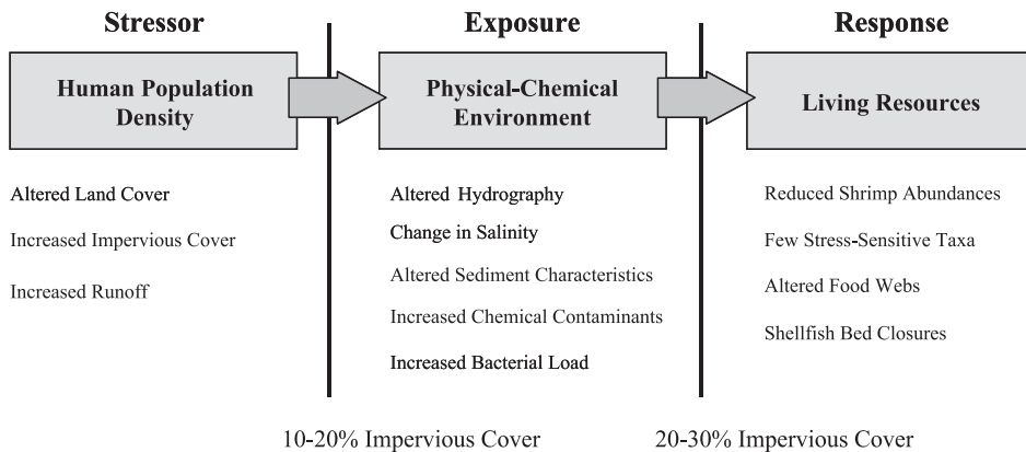
Fig. 5. Summary of the conceptual model of linkages developed for headwater tidal creeks.
