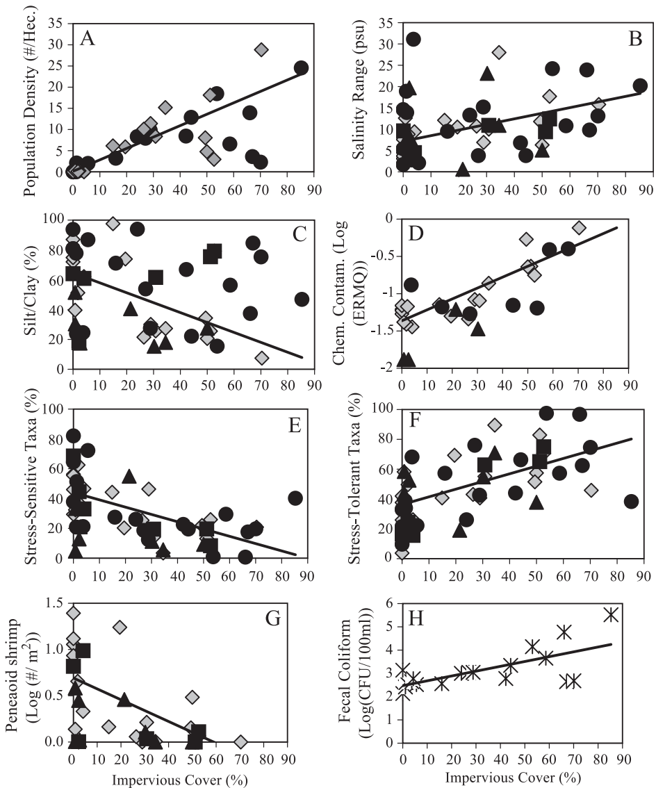
Fig. 3. Comparison of the relationship between eight parameters evaluated in this study and impervious cover (%) for the 1994 summer calibration (diamonds), 1994 summer validation (squares), 1995 summer validation (triangles), 2000 winter calibration (circles), and 2002 summer fecal coliform calibration (asterisks). The line indicates the linear regression for the summer calibration data sets.
