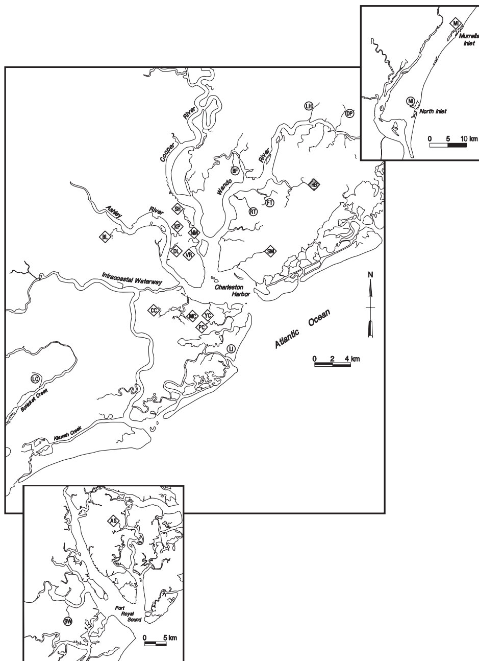
Fig. 1. Map showing location of tidal creeks sampled in South Carolina. The reference (○) and developed/impacted (◊) creeks are presented by their abbreviations (see Table 1). The inserts are the north (top) and south (bottom) sampling sites.
