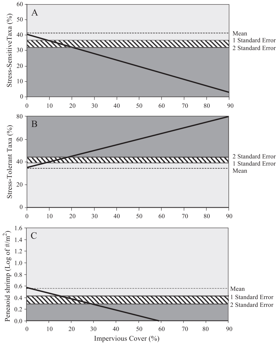
Fig. 6. Diagram of the stress-sensitive (A) and stress-tolerant (B) macrobenthic metrics and the relative abundance of Peneaeid species (C) into three categories based upon the mean of the forested watersheds: (1) good condition (light gray) represented by values that were within one standard error; (2) impacted condition (striped) represented by values that were between one and two standard errors; and (3) degraded condition (dark gray) represented by values that were greater than two standard errors. The regression line for all of the data is also provided.
